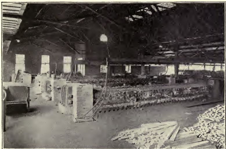
PLATE 11.—Electric Furnaces for Carborundum and Graphite of Acheson Graphite Co., Niagara Falls.
